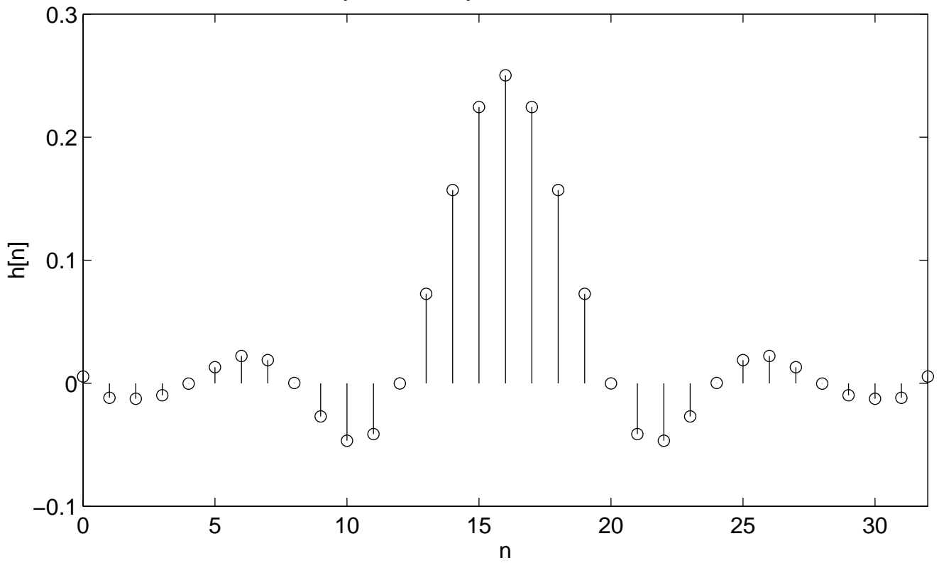
Impulse response of FIR filter
