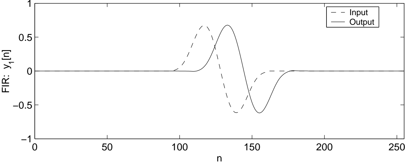
Output of FIR filter
