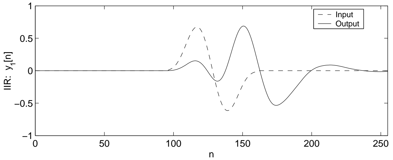
Output of IIR filter
