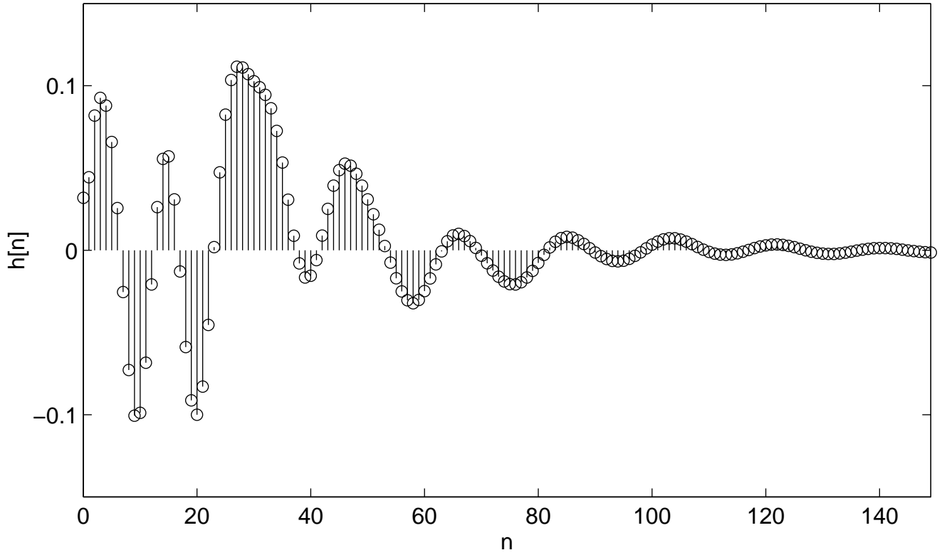
Impulse response of IIR filter
